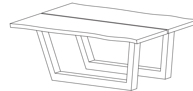
Stol tip 1 | boja postolja: crna, inox izvedba uljene ploče: hrast, orah dimenzije ploče: 1800x1100x750 mm, 2000x1100x750 mm, 2200x1100x750 mm, 2400x1100x750 mm, 2600x1100x750 mm, 2800x1100x750 mm, 3000x1100x750 mm
