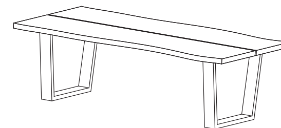
Stol tip 4 | boja postolja: crna, inox izvedba uljene ploče: hrast, orah dimenzije ploče: 1800x1100x750 mm, 2000x1100x750 mm, 2200x1100x750 mm, 2400x1100x750 mm, 2600x1100x750 mm, 2800x1100x750 mm, 3000x1100x750 mm
