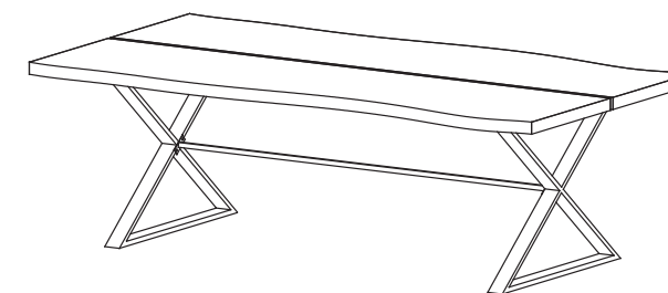
Stol tip 2 | boja postolja: crna, inox izvedba uljene ploče: hrast, orah dimenzije ploče: 1800x1100x750 mm, 2000x1100x750 mm, 2200x1100x750 mm, 2400x1100x750 mm, 2600x1100x750 mm, 2800x1100x750 mm, 3000x1100x750 mm
